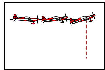
Fig. 58 The horizontal flight path should be maintained until the spin starts.
